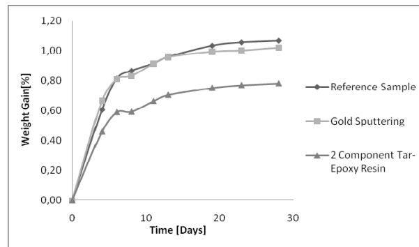
Fig. 7: Saturation curve of the coated fleece samples in a water basin (T = 23 °C).
