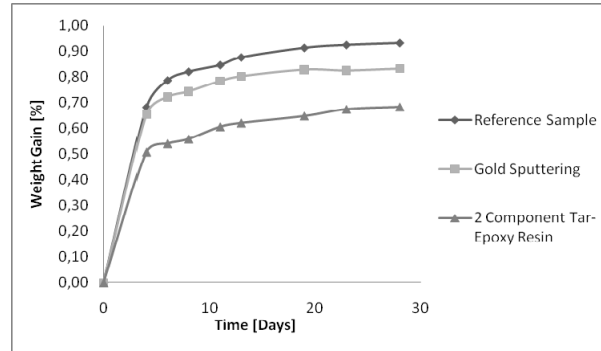
Fig. 6: Saturation curve of the coated fleece samples in a water basin (T = 50 °C).
