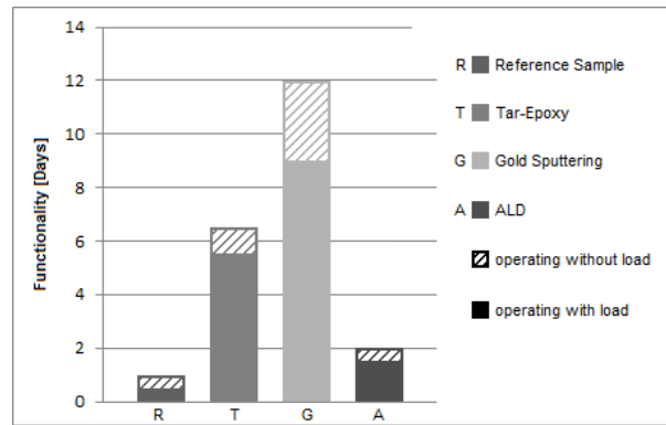
Fig. 8: Underwater service life of actuators with and without load.
