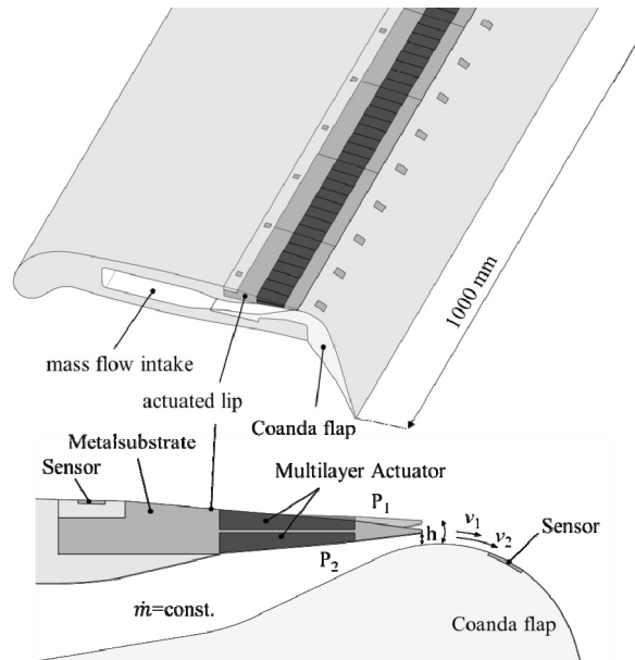
Fig. 1: Concept of the actuated slot-lip for water tunnel tests [1].
