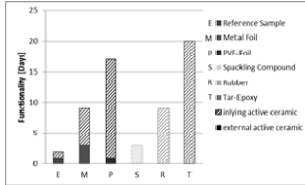
Fig. 10: Underwater service life of the slot-lip.
