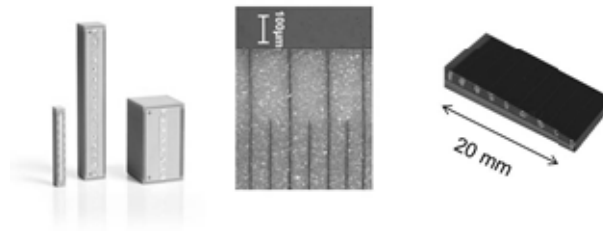
Fig. 9: left: Commercial multilayer actuators, middle: Multilayer microsection with electrodes, right: customized actuator.
